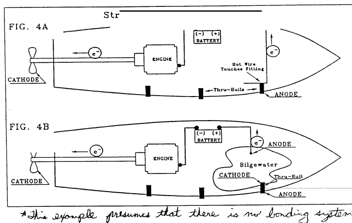
Figure C: Stray Current Corrosion
