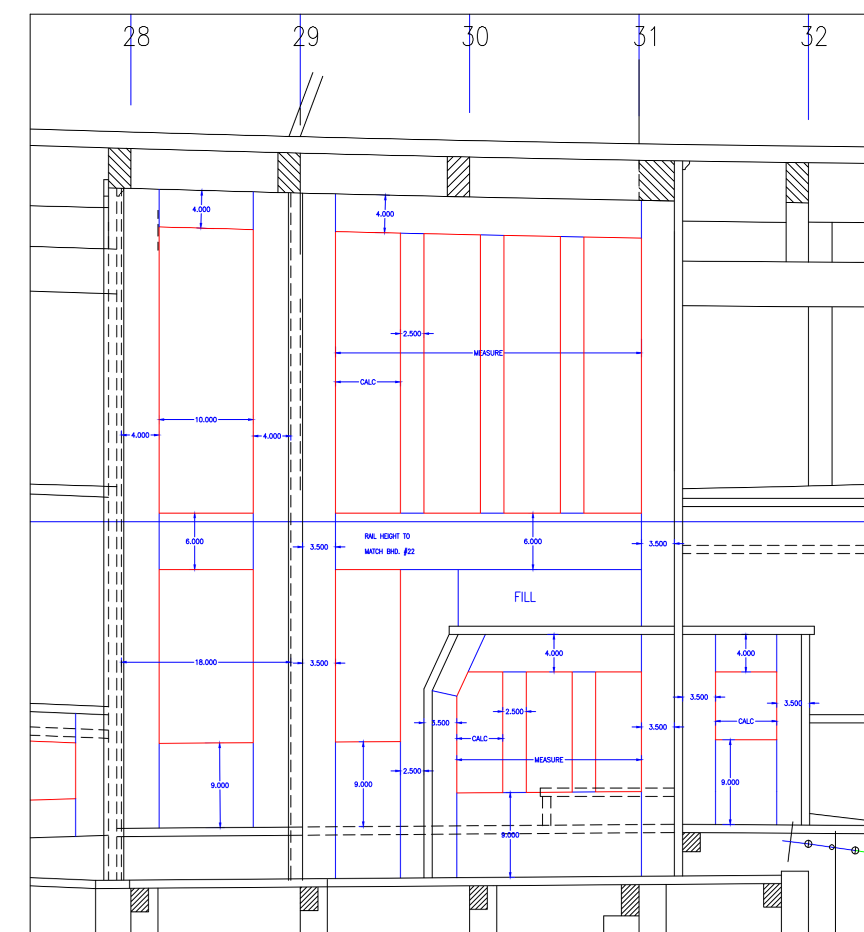
FORE-AND-AFT BULKHEAD AND DOOR FOR MAIN HEAD ENGINE BOX PORT-SIDE PANELS LOOKING TO STARBOARD IN MAIN PASSAGEWAY
