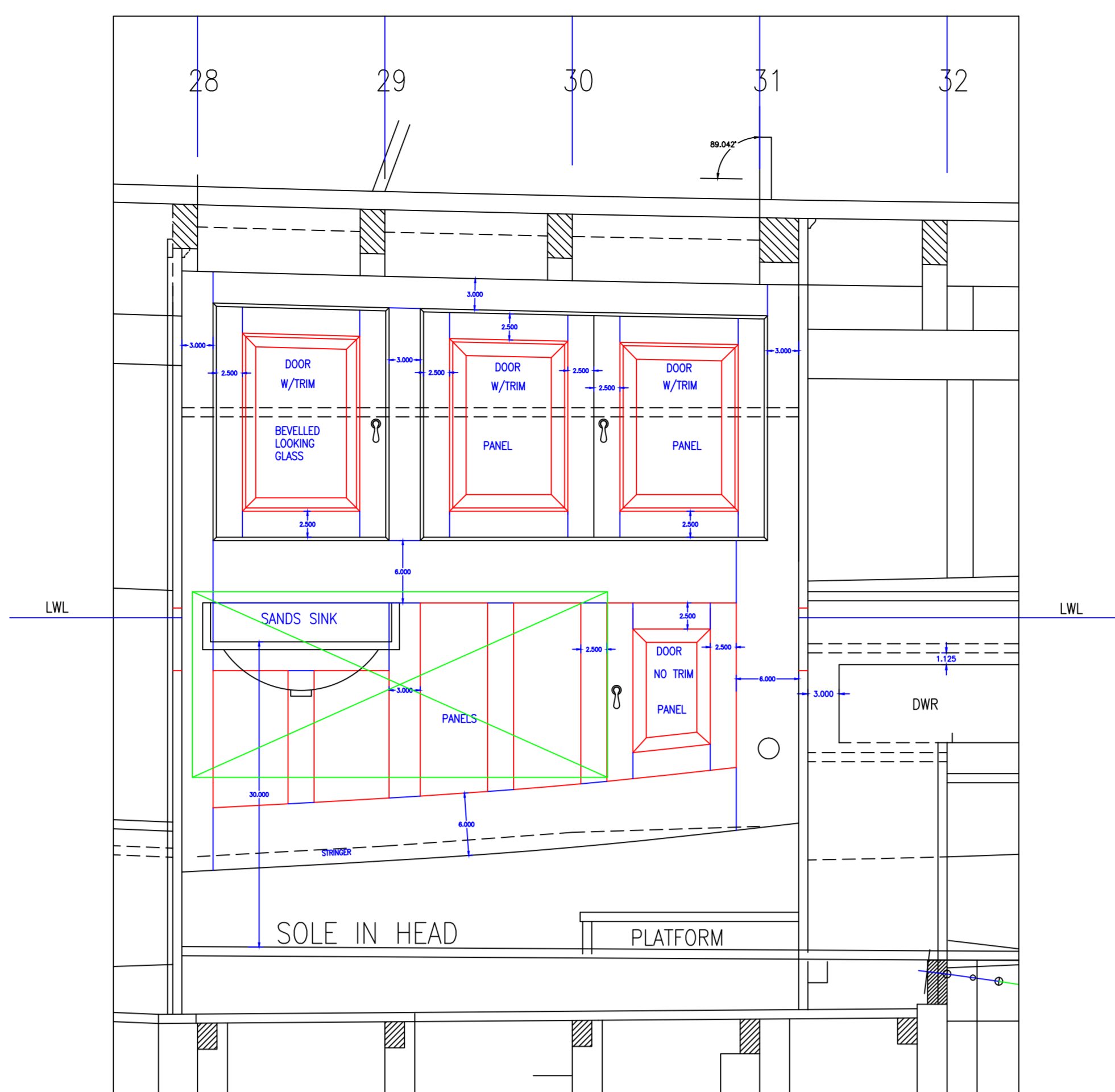
FINAL HEAD PANEL LAYOUT
