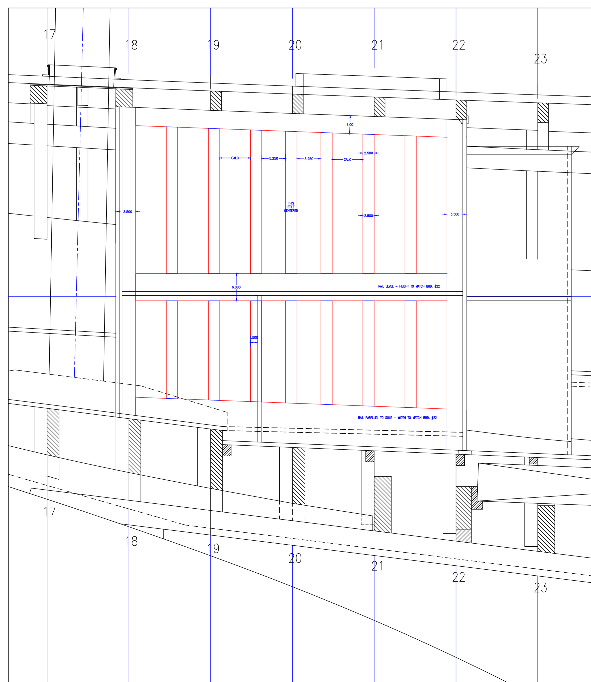
FORE-AND-AFT BULKHEAD BETWEEN GALLEY AND CAPT. CABIN
