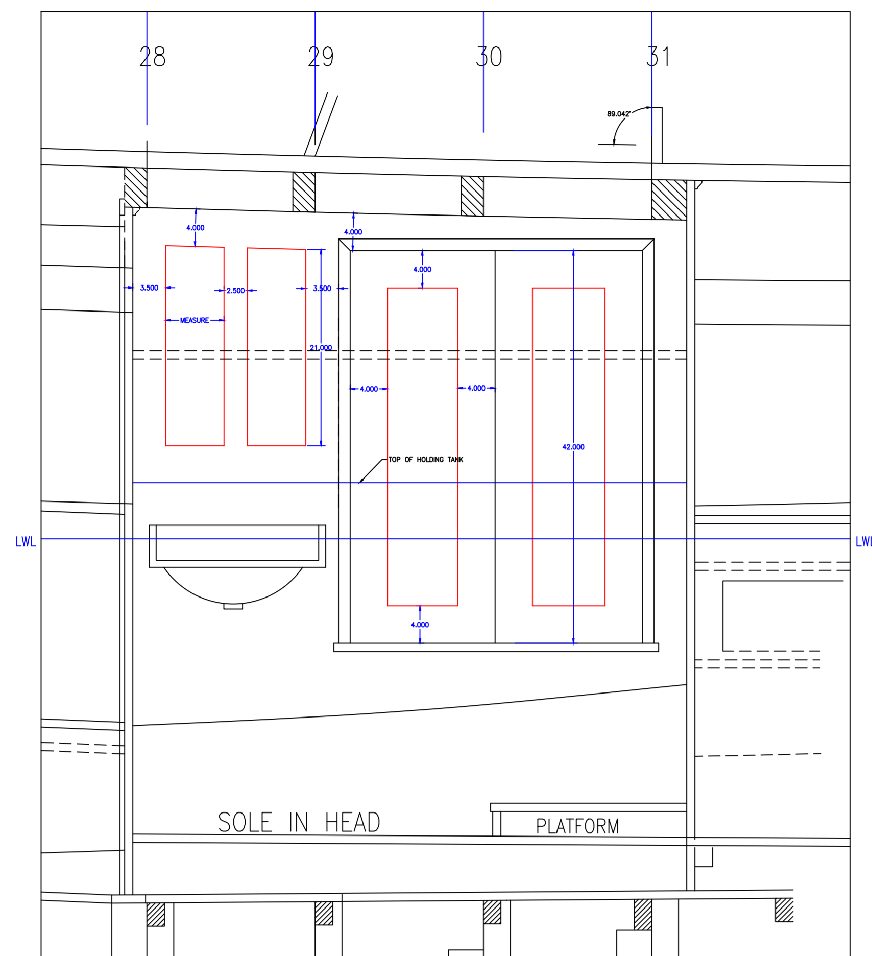
ORIGINAL HEAD PANEL LAYOUT
