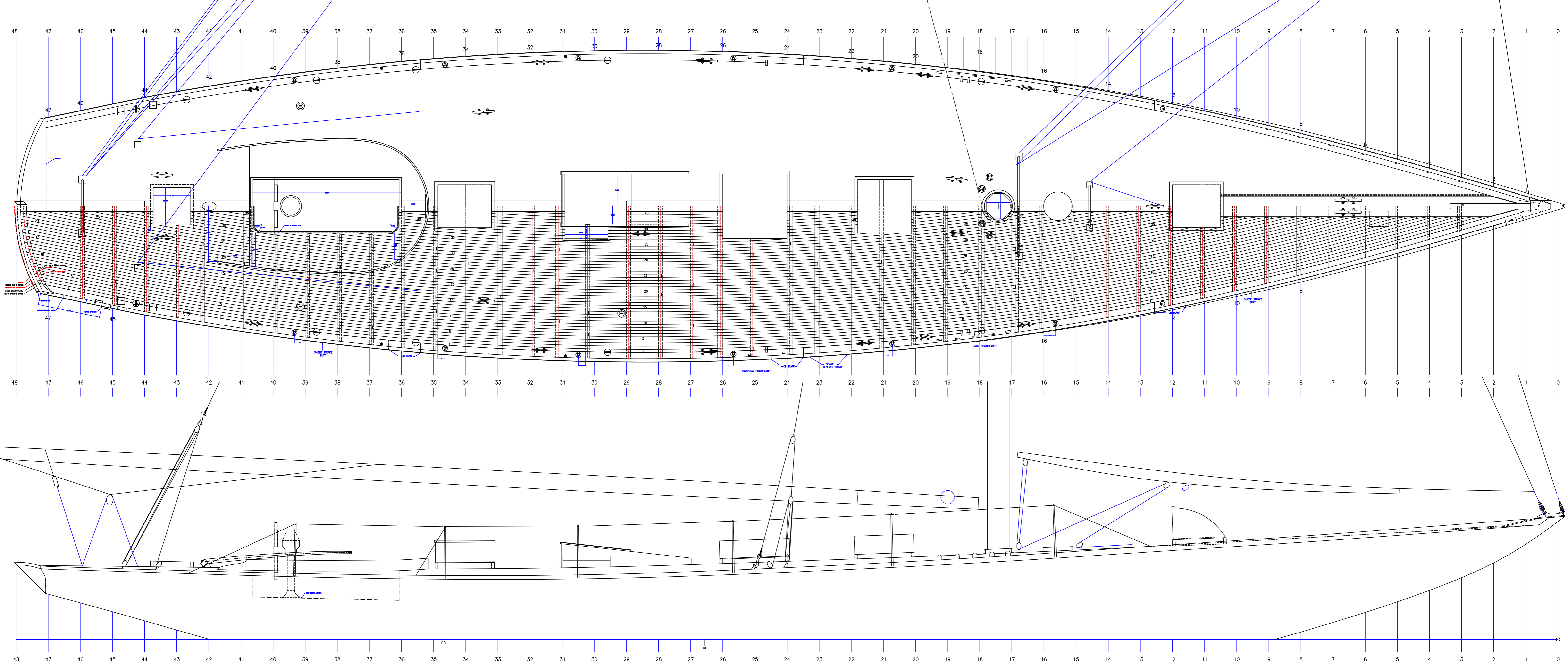
SPARTAN DECK HARDWARE LAYOUT MP&G
